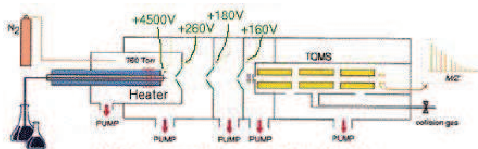
a) Electro-spray ion cluster analyzing system
