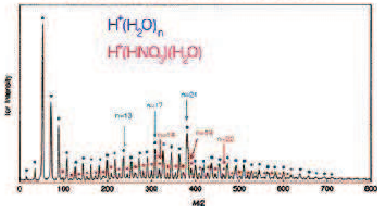
b) Mass spectra of ion clusters derived from aqueous solution of nitric acid
