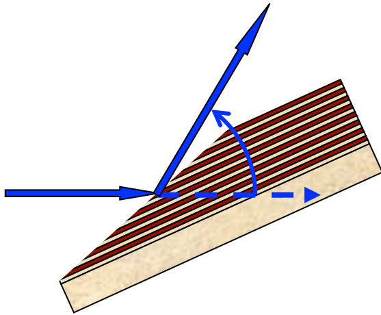
Asymmetric cut multilayers act as dispersive gratings.
