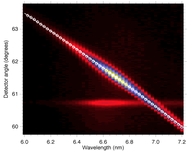
Measured dispersion from asymmetric cut multilayer (grating)
