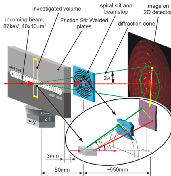
Figure 5.19: Spiral slit geometry. Only small fractions of individual diffraction rings are transmitted but independently of the crystal symmetry (Martins & Honkimäki, 2003).
