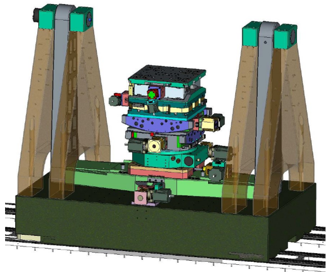
Figure 5.12: The interface diffractometer and key performance parameters. The order of components in the table reflects their vertical arrangement (courtesy by Huber).
