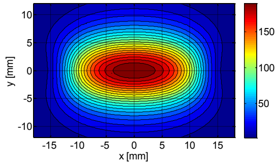
Figure 2.3: Power density distribution of a 2.1 cm period in-vacuum undulator. The distance from the source is 100 m and units are kW/mrad 2 .
